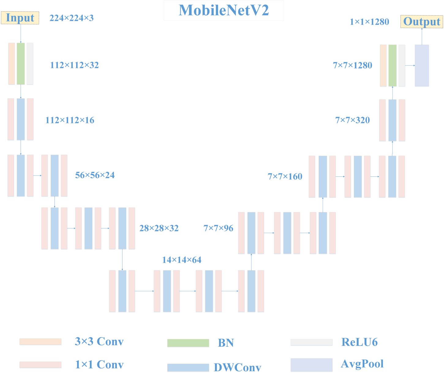
Figure 1. from Wenna Cai et al 2026 Astron. J. 171 doi:10.3847/1538-3881/ae2ad5 https://dx.doi.org/10.3847/1538-3881/ae2ad5 © 2026. The Author(s). Published by the American Astronomical Society.
