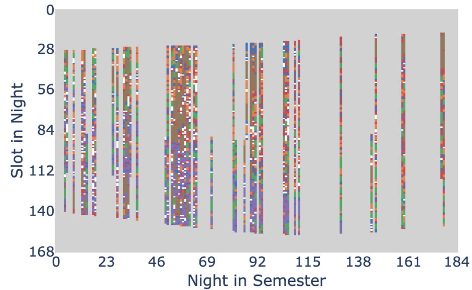
Figure 5. from Jack Lubin et al 2026 Astron. J. 171 doi:10.3847/1538-3881/ae2a2e https://dx.doi.org/10.3847/1538-3881/ae2a2e © 2026. The Author(s). Published by the American Astronomical Society.
