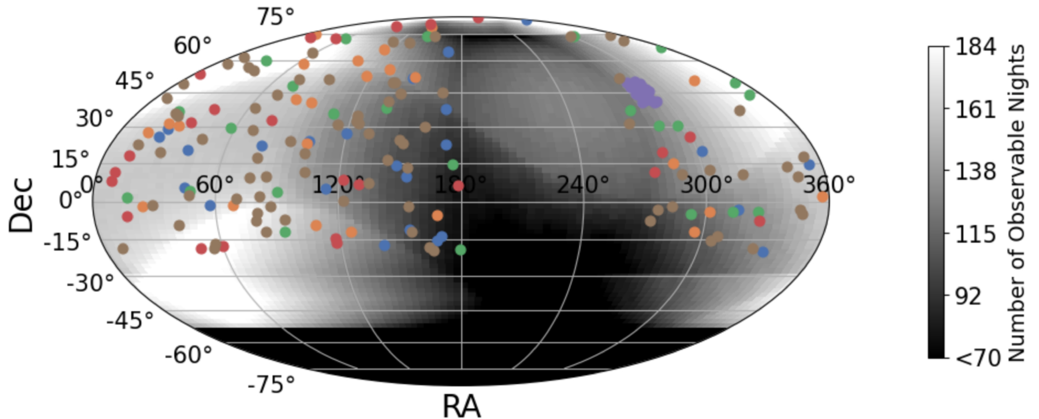
Figure 4. from Jack Lubin et al 2026 Astron. J. 171 doi:10.3847/1538-3881/ae2a2e https://dx.doi.org/10.3847/1538-3881/ae2a2e © 2026. The Author(s). Published by the American Astronomical Society.
