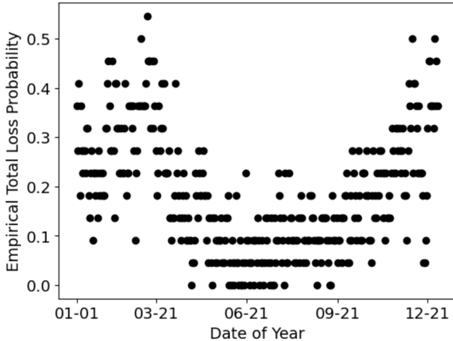
Figure 3. from Jack Lubin et al 2026 Astron. J. 171 doi:10.3847/1538-3881/ae2a2e https://dx.doi.org/10.3847/1538-3881/ae2a2e © 2026. The Author(s). Published by the American Astronomical Society.
