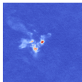
Ground Truth G34.30 SPW 27 Ch. 320
