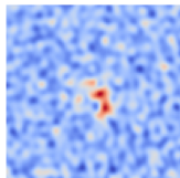
Ground Truth LkCa 15 Setting A SPW 3 Ch. 1571
