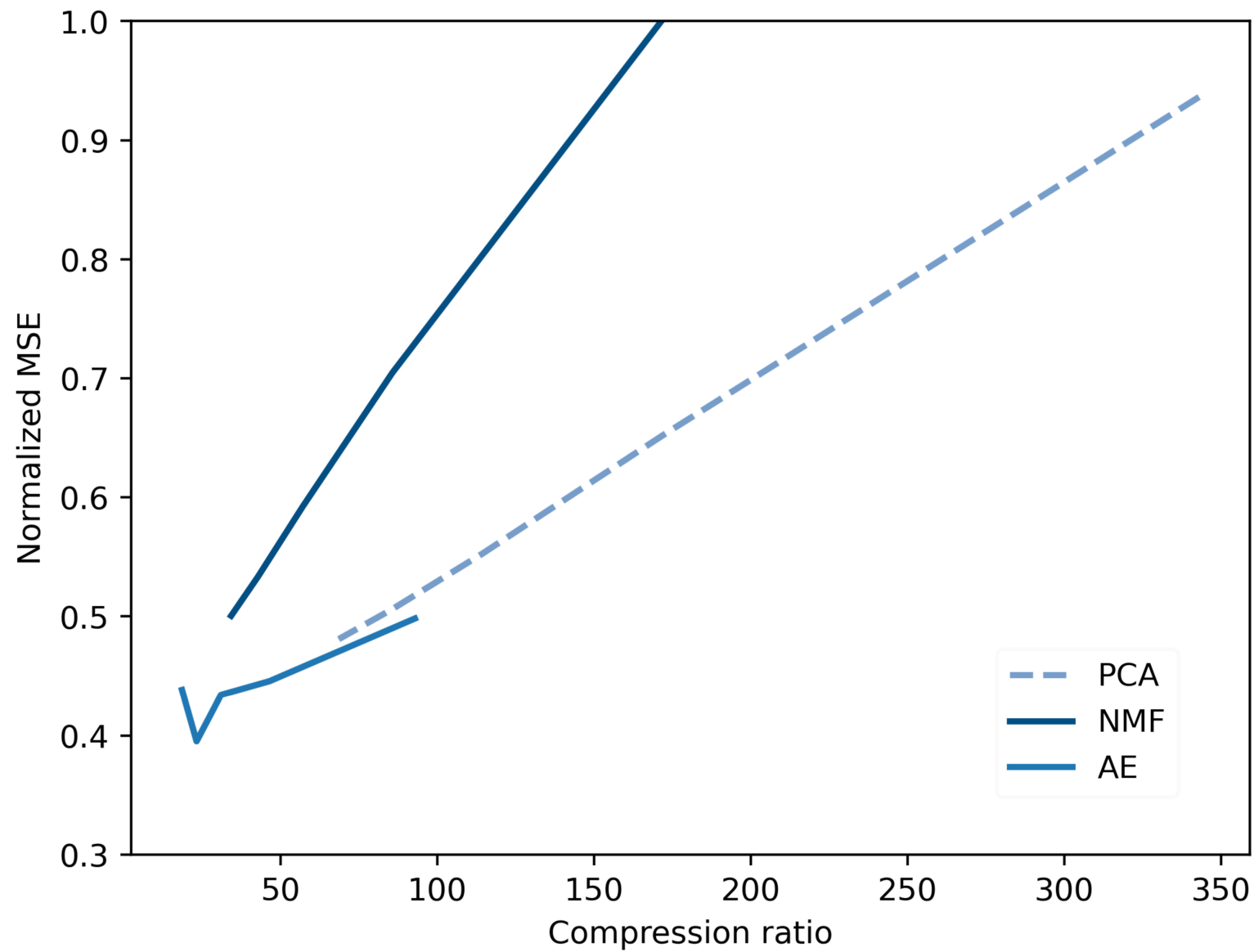
Figure 7. from Haley N. Scolati et al 2026 Astron. J. 171 doi:10.3847/1538-3881/ae2a06 https://dx.doi.org/10.3847/1538-3881/ae2a06 © 2026. The Author(s). Published by the American Astronomical Society.
