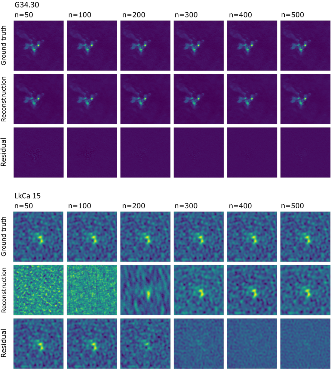
Figure 10. from Haley N. Scolati et al 2026 Astron. J. 171 doi:10.3847/1538-3881/ae2a06 https://dx.doi.org/10.3847/1538-3881/ae2a06 © 2026. The Author(s). Published by the American Astronomical Society.
