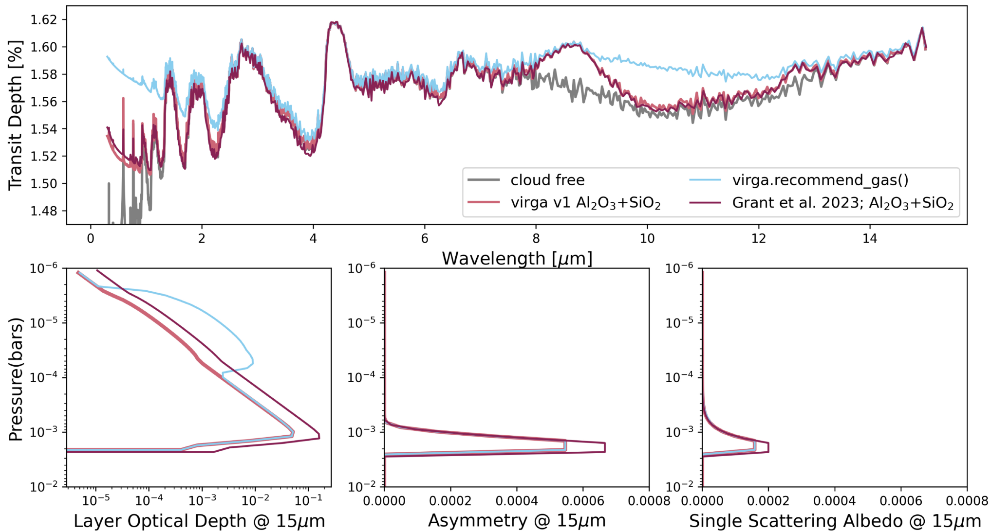
Figure 9. from Natasha E. Batalha et al 2026 Astron. J. 171 doi:10.3847/1538-3881/ae29e5 https://dx.doi.org/10.3847/1538-3881/ae29e5 © 2026. The Author(s). Published by the American Astronomical Society.
