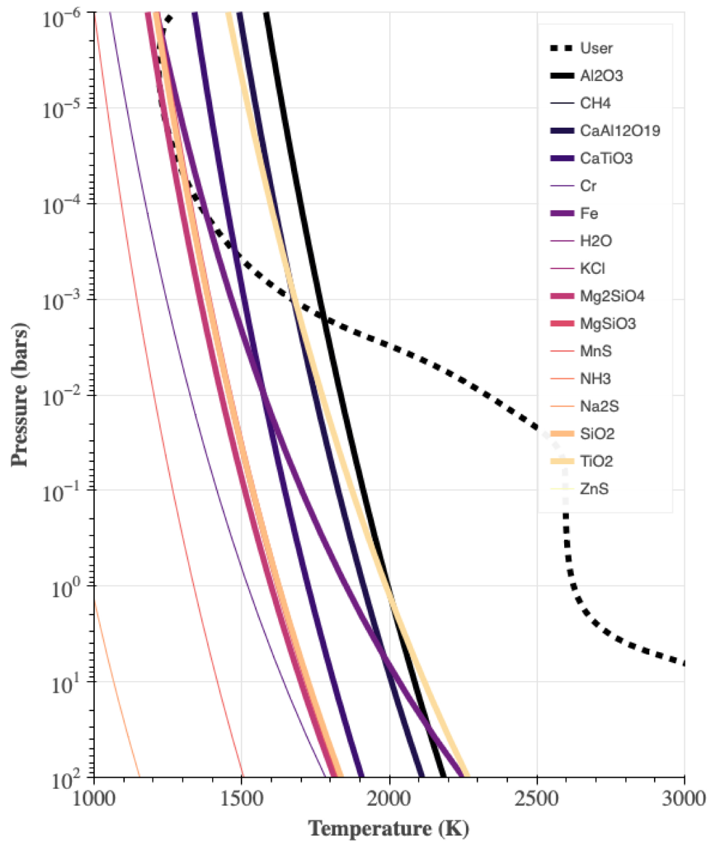
Figure 8. from Natasha E. Batalha et al 2026 Astron. J. 171 doi:10.3847/1538-3881/ae29e5 https://dx.doi.org/10.3847/1538-3881/ae29e5 © 2026. The Author(s). Published by the American Astronomical Society.
