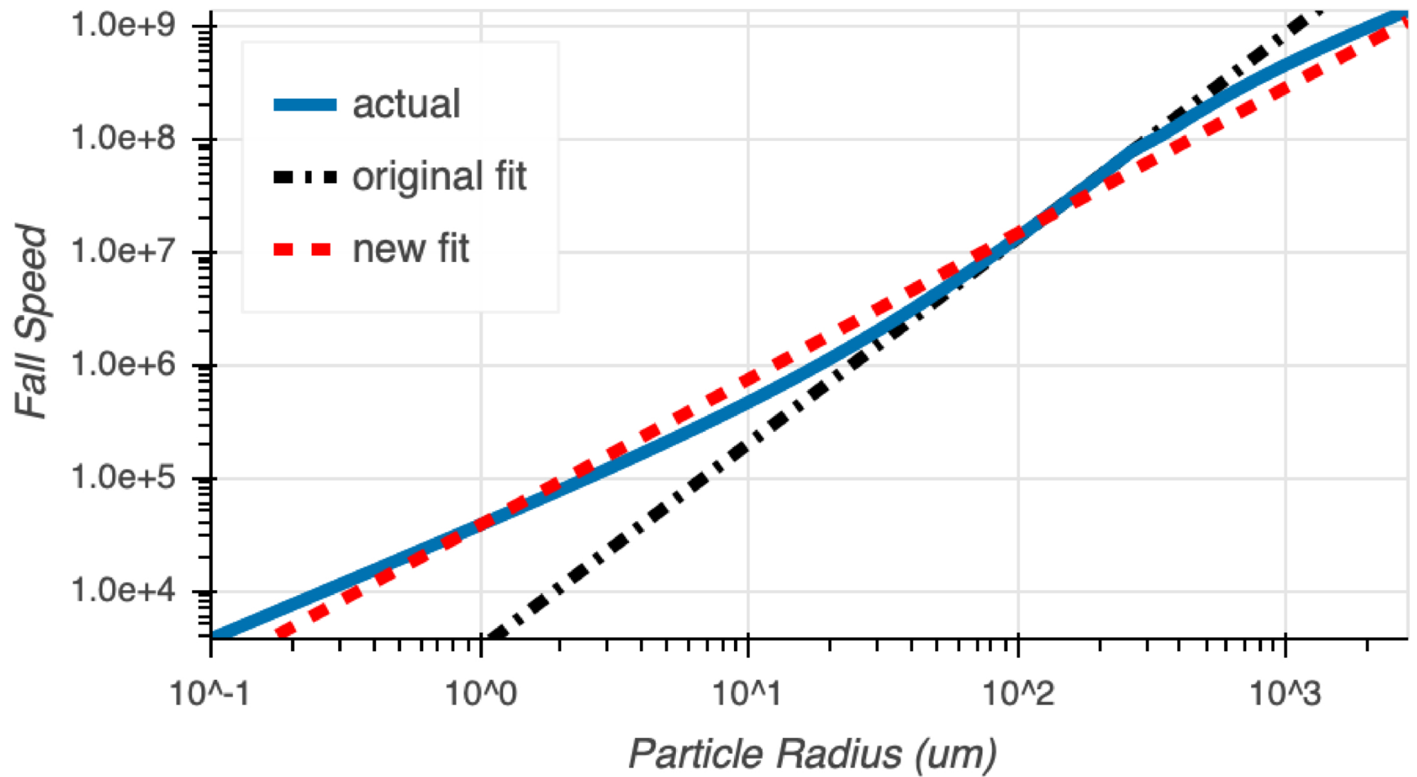
Figure 7. from Natasha E. Batalha et al 2026 Astron. J. 171 doi:10.3847/1538-3881/ae29e5 https://dx.doi.org/10.3847/1538-3881/ae29e5 © 2026. The Author(s). Published by the American Astronomical Society.
