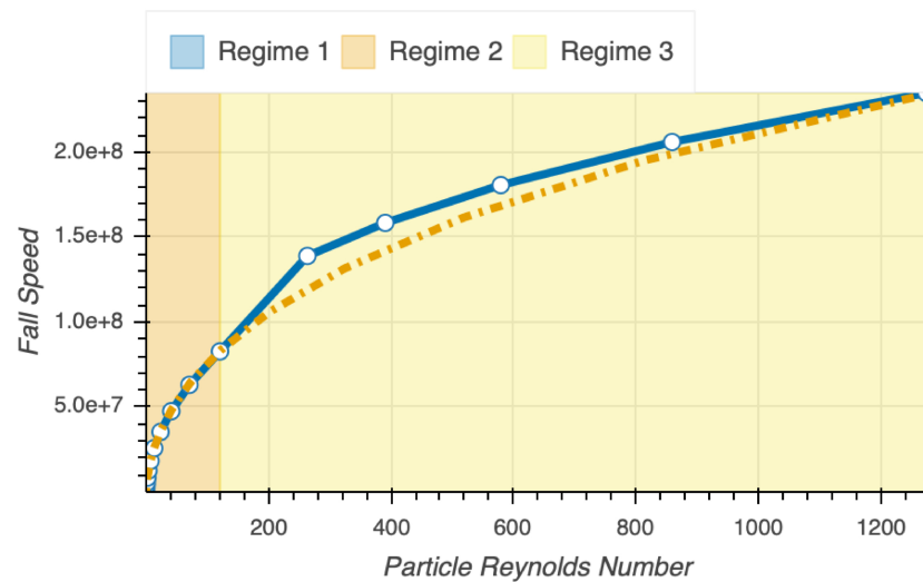
(b) 10 bars
