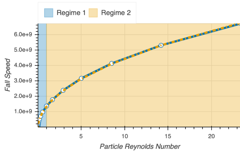
(a) 10^{-4} bars
