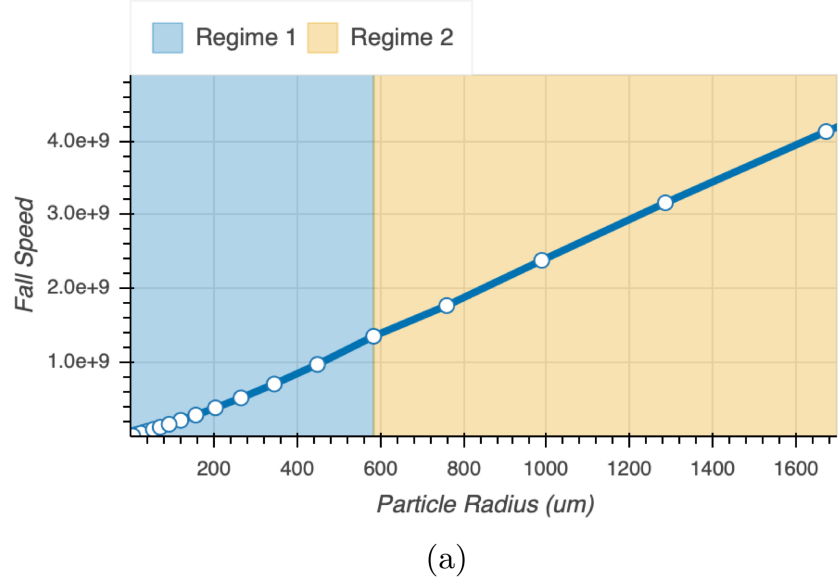
Figure 5. from Natalsha E. Batalha et al 2026 Astron. J. 171 doi:10.3847/1538-3881/ae29e5 https://dx.doi.org/10.3847/1538-3881/ae29e5 © 2026. The Author(s). Published by the American Astronomical Society.
