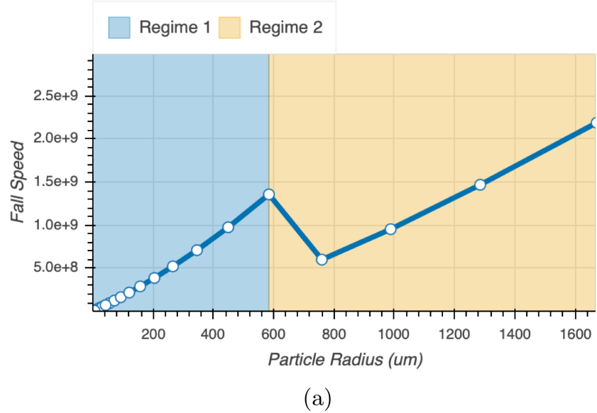
Figure 3. from Natasha E. Batalha et al 2026 Astron. J. 171 doi:10.3847/1538-3881/ae29e5 https://dx.doi.org/10.3847/1538-3881/ae29e5 © 2026. The Author(s). Published by the American Astronomical Society.
