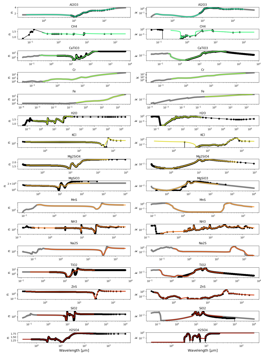
Figure 2. from Natasha E. Batalha et al 2026 Astron. J. 171 doi:10.3847/1538-3881/ae29e5 https://dx.doi.org/10.3847/1538-3881/ae29e5 © 2026. The Author(s). Published by the American Astronomical Society.
