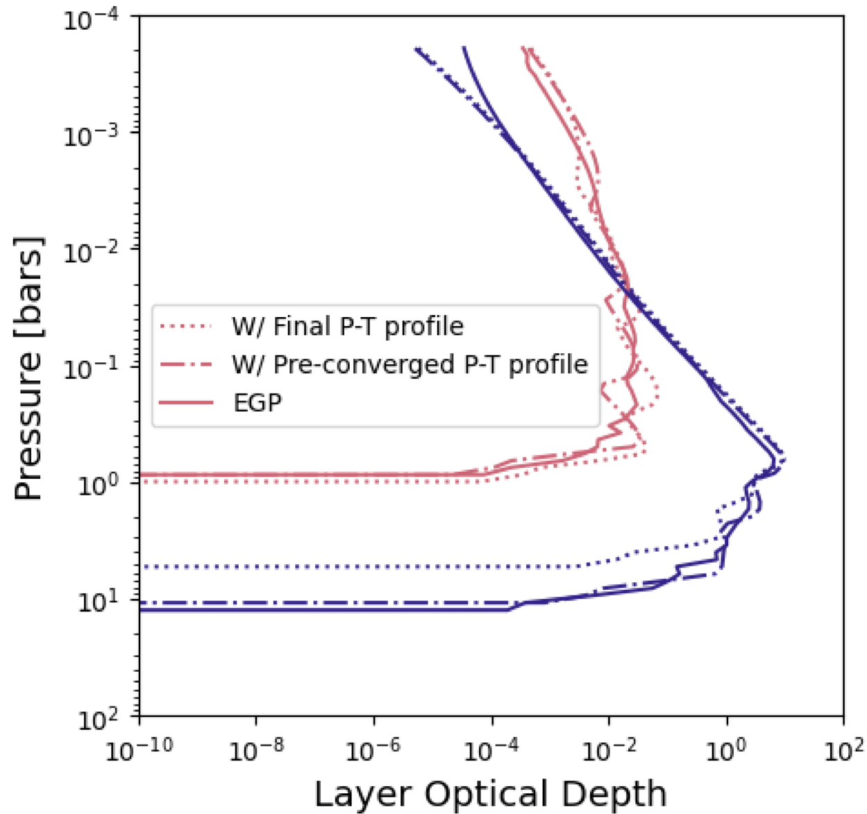
Figure 11. from Natasha E. Batalha et al 2026 Astron. J. 171 doi:10.3847/1538-3881/ae29e5 https://dx.doi.org/10.3847/1538-3881/ae29e5 © 2026. The Author(s). Published by the American Astronomical Society.
