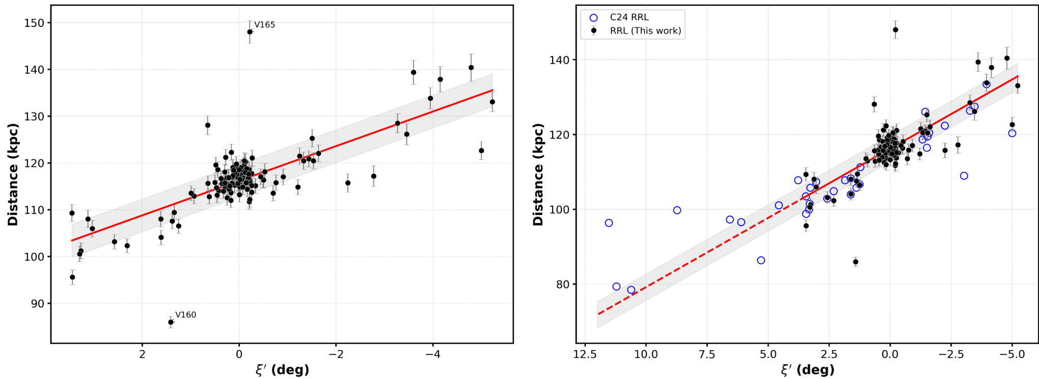
Figure 8. from A. Katherina Vivas et al 2026 Astron. J. 171 doi:10.3847/1538-3881/ae29a8 https://dx.doi.org/10.3847/1538-3881/ae29a8 © 2026. The Author(s). Published by the American Astronomical Society.
