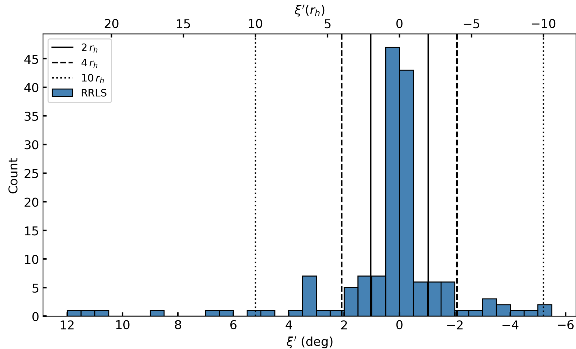
Figure 7. from A. Katherina Vivas et al 2026 Astron. J. 171 doi:10.3847/1538-3881/ae29a8 https://dx.doi.org/10.3847/1538-3881/ae29a8 © 2026. The Author(s). Published by the American Astronomical Society.
