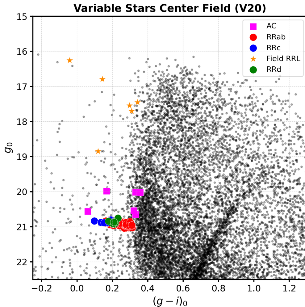
Figure 4. from A. Katherina Vivas et al 2026 Astron. J. 171 doi:10.3847/1538-3881/ae29a8 https://dx.doi.org/10.3847/1538-3881/ae29a8 © 2026. The Author(s). Published by the American Astronomical Society.
