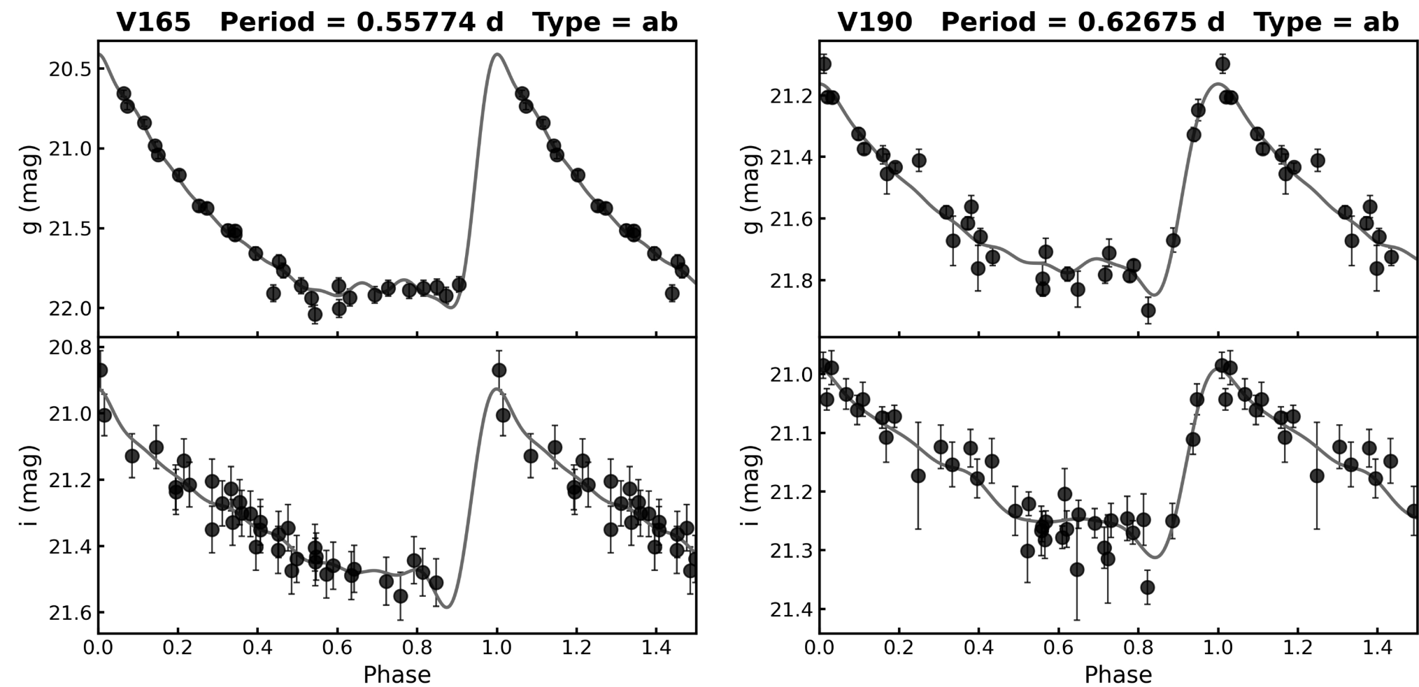
Figure 2. Lightcurves from A. Katherina Vivas et al 2026 Astron. J. 171 doi:10.3847/1538-3881/ae29a8 https://dx.doi.org/10.3847/1538-3881/ae29a8 © 2026. The Author(s). Published by the American Astronomical Society.
