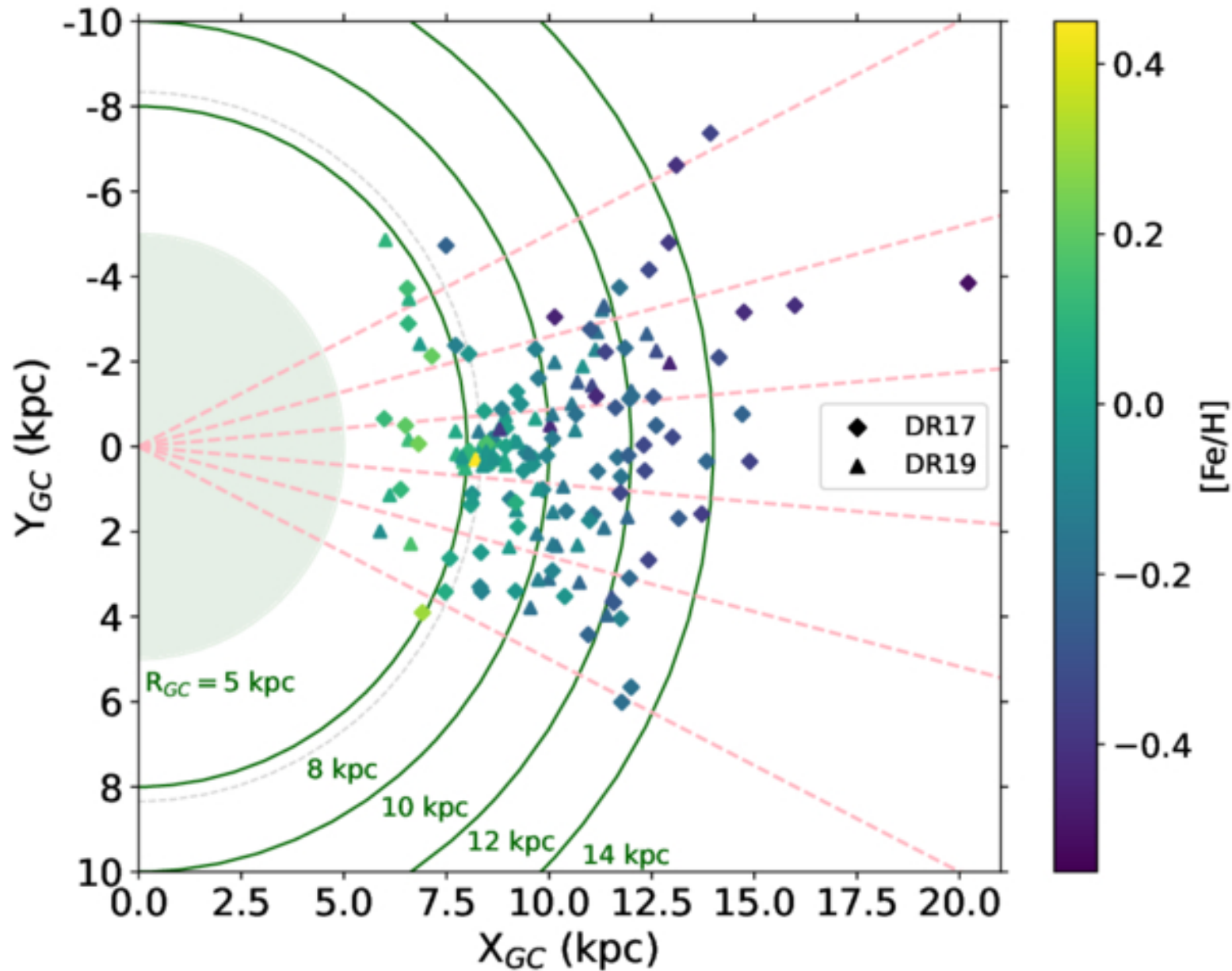
Figure 8. from Jonah M. Otto et al 2026 Astron. J. 171 doi:10.3847/1538-3881/ae28d8 https://dx.doi.org/10.3847/1538-3881/ae28d8 © 2026. The Author(s). Published by the American Astronomical Society.
