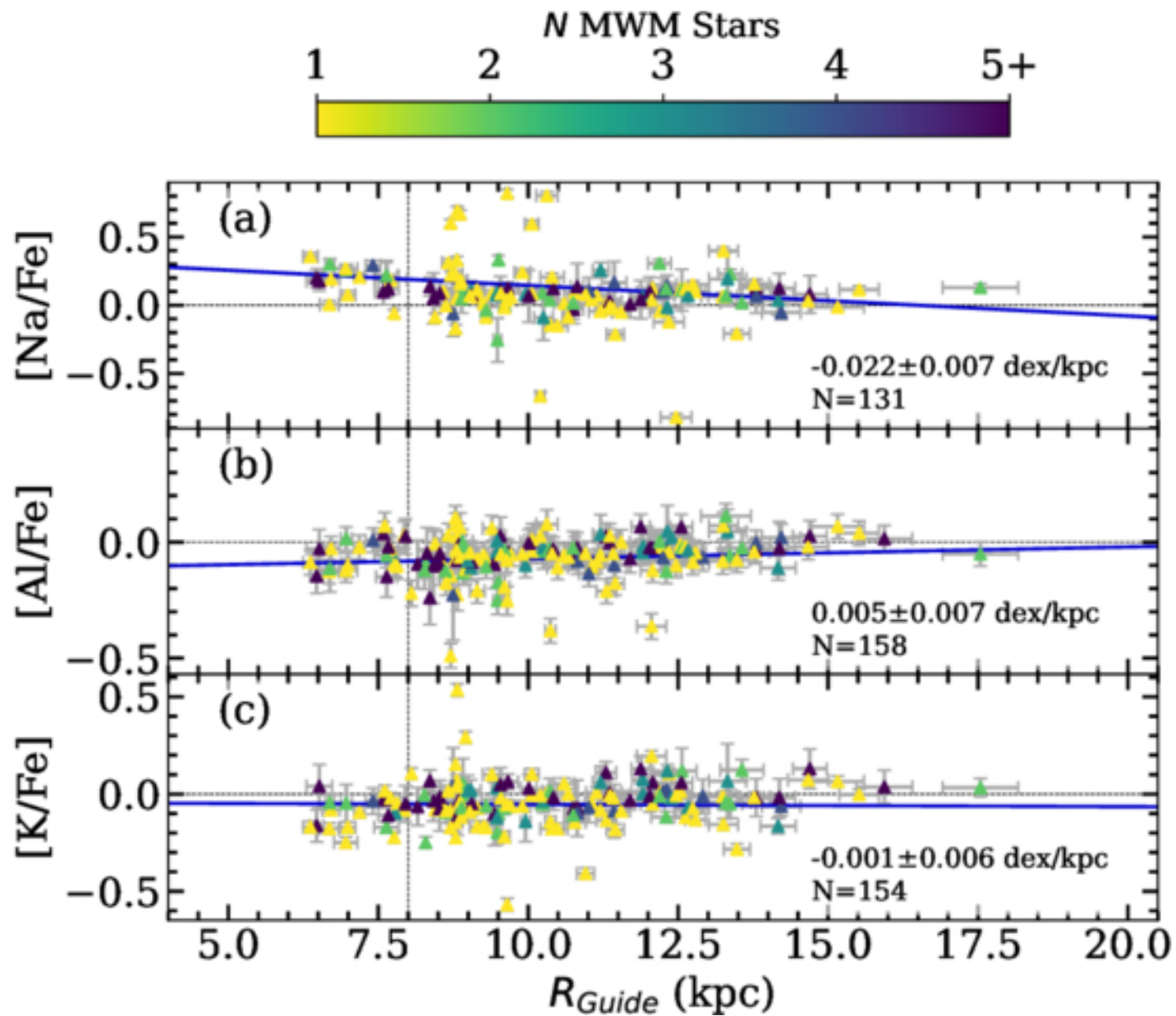
Figure 6. from Jonah M. Otto et al 2026 Astron. J. 171 doi:10.3847/1538-3881/ae28d8 https://dx.doi.org/10.3847/1538-3881/ae28d8 © 2026. The Author(s). Published by the American Astronomical Society.
