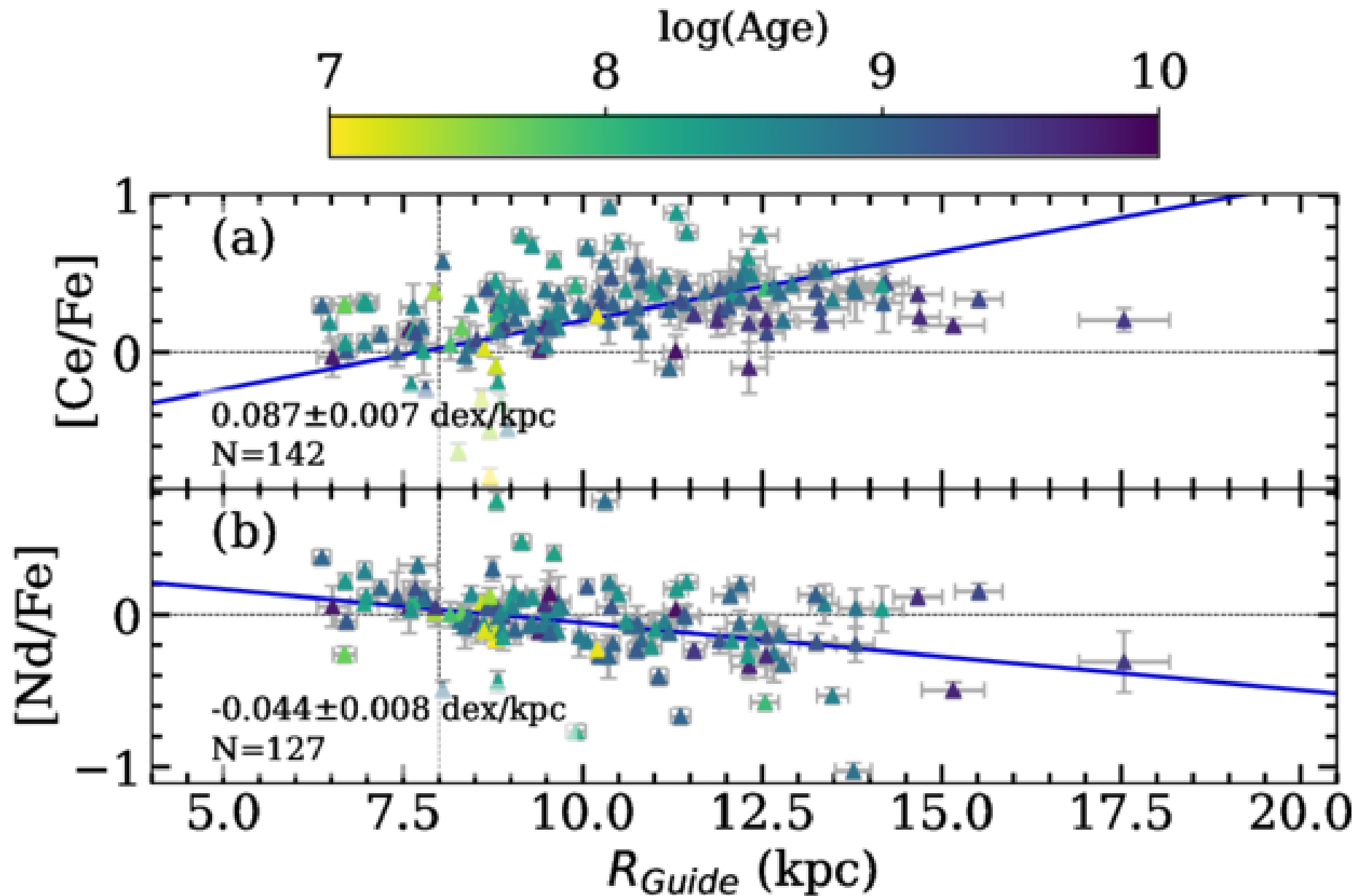
Figure 26. from Jonah M. Otto et al 2026 Astron. J. 171 doi:10.3847/1538-3881/ae28d8 https://dx.doi.org/10.3847/1538-3881/ae28d8 © 2026. The Author(s). Published by the American Astronomical Society.
