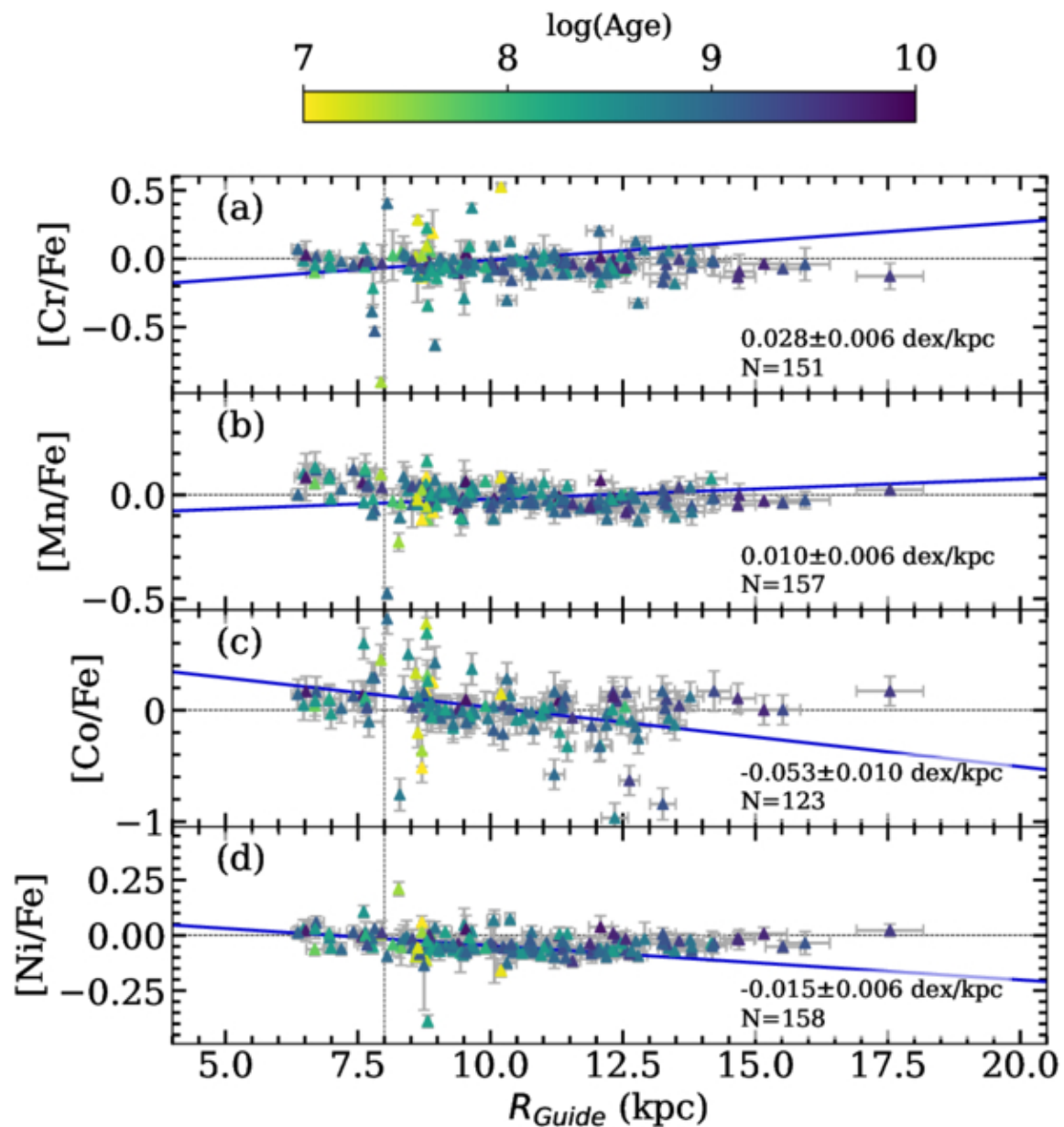
Figure 24. from Jonah M. Otto et al 2026 Astron. J. 171 doi:10.3847/1538-3881/ae28d8 https://dx.doi.org/10.3847/1538-3881/ae28d8 © 2026. The Author(s). Published by the American Astronomical Society.
