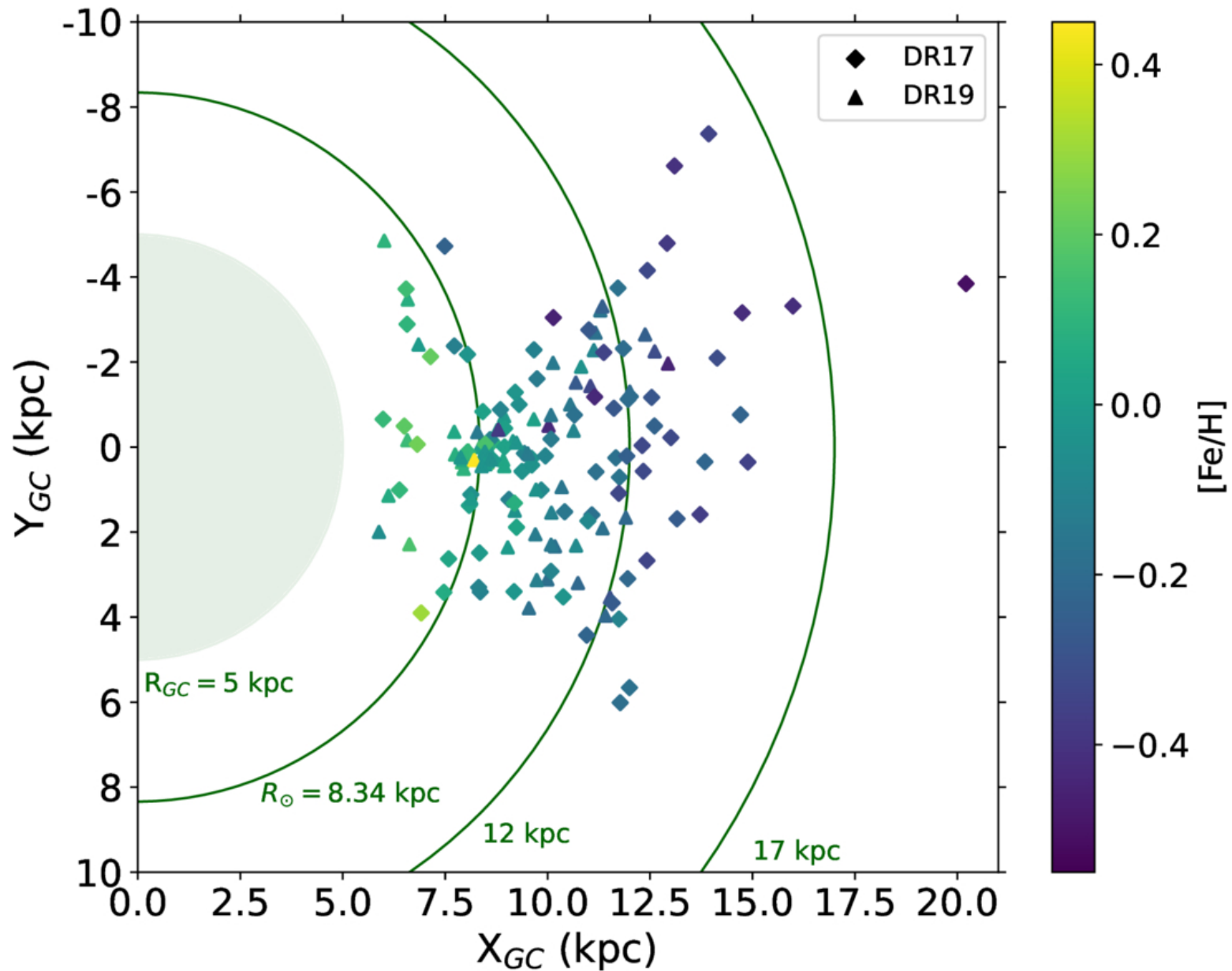
Figure 2. from Jonah M. Otto et al 2026 Astron. J. 171 doi:10.3847/1538-3881/ae28d8 https://dx.doi.org/10.3847/1538-3881/ae28d8 © 2026. The Author(s). Published by the American Astronomical Society.
