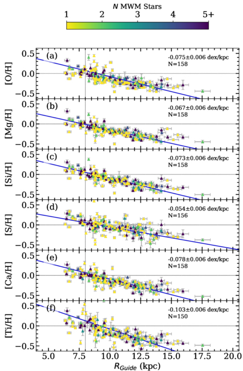
Figure 19. from Jonah M. Otto et al 2026 Astron. J. 171 doi:10.3847/1538-3881/ae28d8 https://dx.doi.org/10.3847/1538-3881/ae28d8 © 2026. The Author(s). Published by the American Astronomical Society.
