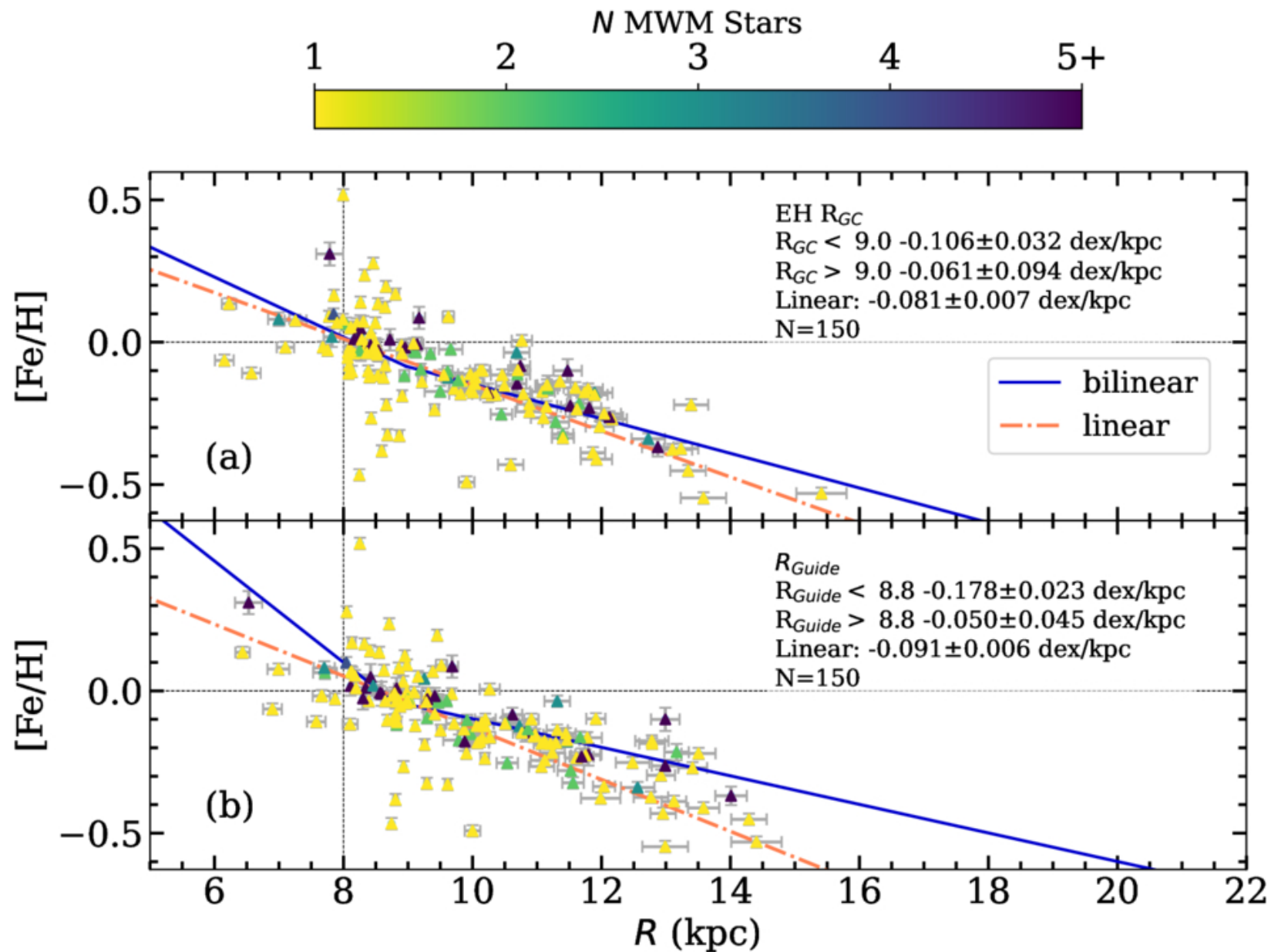
Figure 18. from Jonah M. Otto et al 2026 Astron. J. 171 doi:10.3847/1538-3881/ae28d8 https://dx.doi.org/10.3847/1538-3881/ae28d8 © 2026. The Author(s). Published by the American Astronomical Society.
