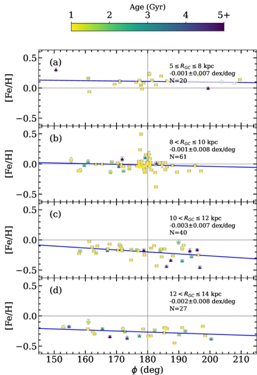
Figure 10. from Jonah M. Otto et al 2026 Astron. J. 171 doi:10.3847/1538-3881/ae28d8 https://dx.doi.org/10.3847/1538-3881/ae28d8 © 2026. The Author(s). Published by the American Astronomical Society.
