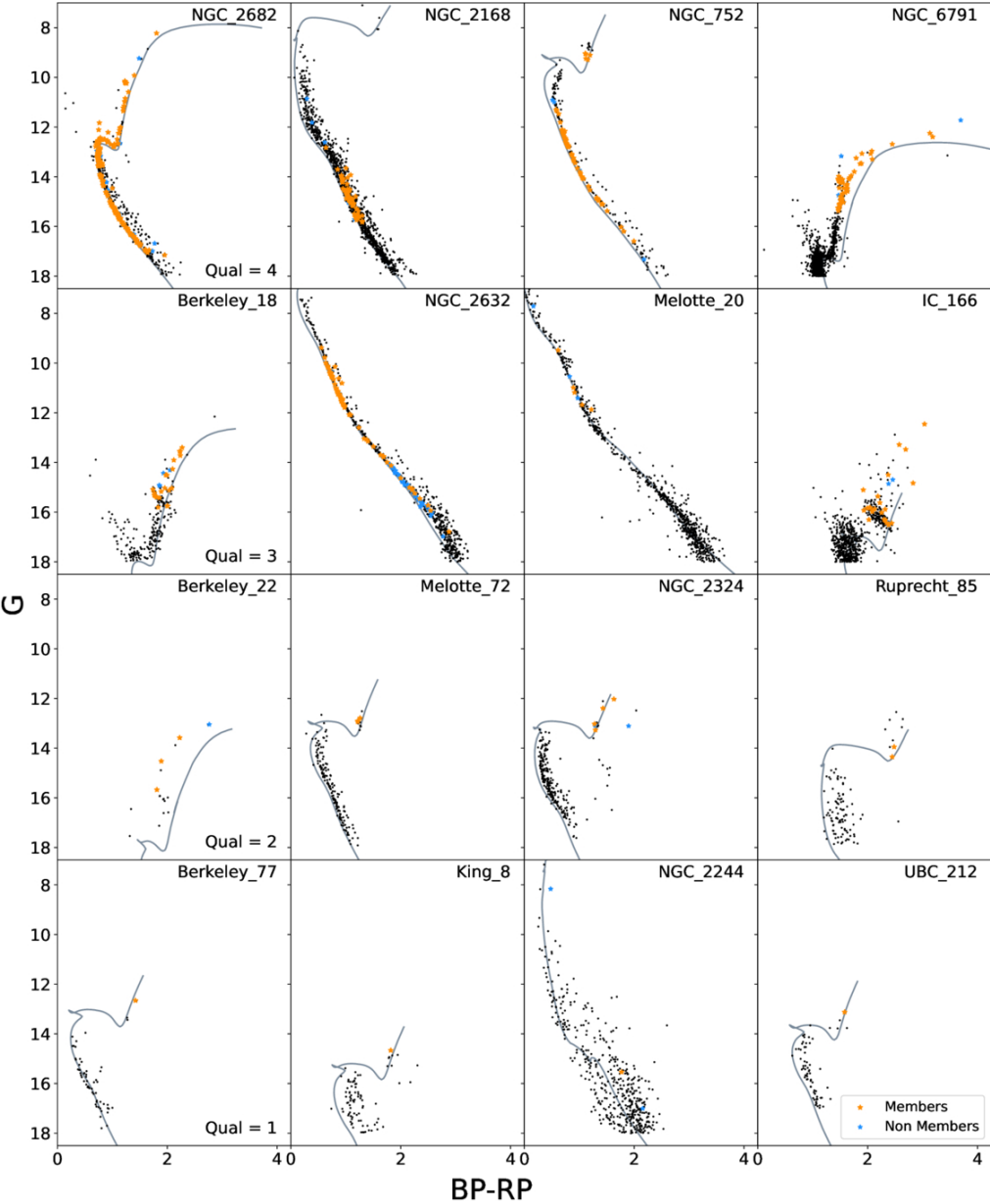
Figure 1. from Jonah M. Otto et al 2026 Astron. J. 171 doi:10.3847/1538-3881/ae28d8 https://dx.doi.org/10.3847/1538-3881/ae28d8 © 2026. The Author(s). Published by the American Astronomical Society.
