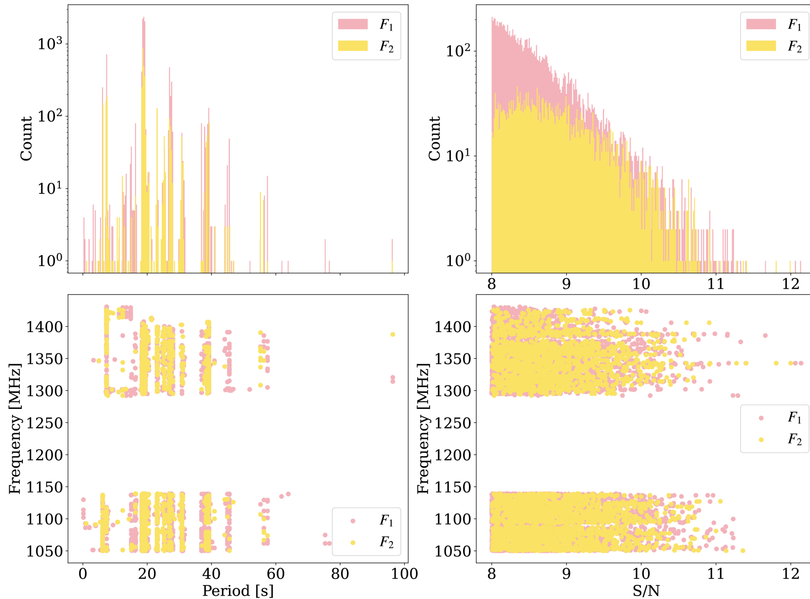
Figure 8. from Jian-Kang Li et al 2026 Astron. J. 171 doi:10.3847/1538-3881/ae28cc https://dx.doi.org/10.3847/1538-3881/ae28cc © 2026. The Author(s). Published by the American Astronomical Society.
