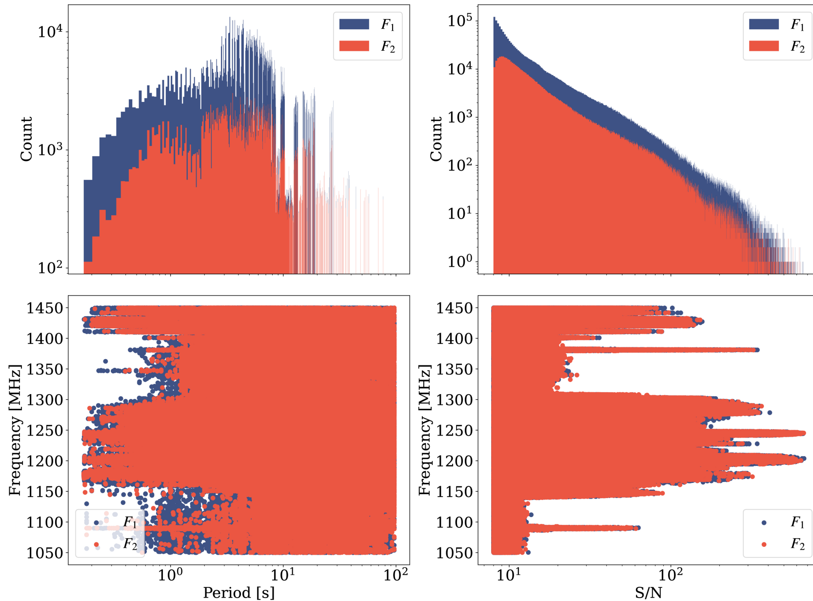
Figure 7. from Jian-Kang Li et al 2026 Astron. J. 171 doi:10.3847/1538-3881/ae28cc https://dx.doi.org/10.3847/1538-3881/ae28cc © 2026. The Author(s). Published by the American Astronomical Society.
