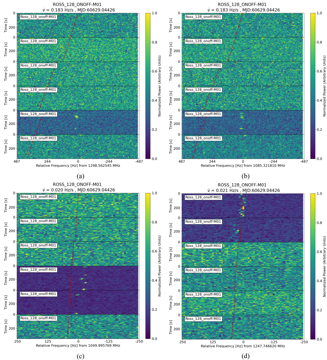
Figure 6. from Jian-Kang Li et al 2026 Astron. J. 171 doi:10.3847/1538-3881/ae28cc https://dx.doi.org/10.3847/1538-3881/ae28cc © 2026. The Author(s). Published by the American Astronomical Society.
