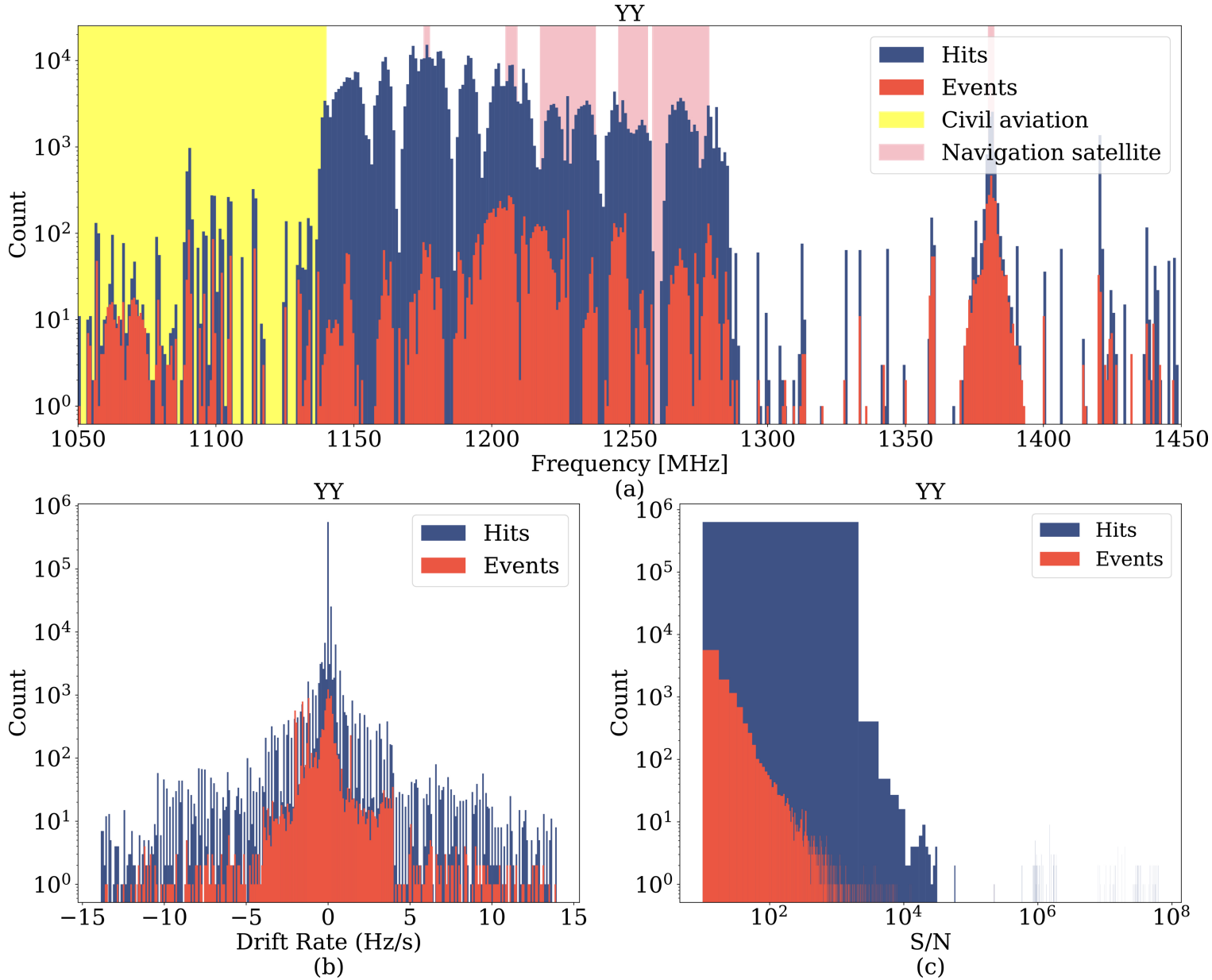
Figure 5. from Jian-Kang Li et al 2026 Astron. J. 171 doi:10.3847/1538-3881/ae28cc https://dx.doi.org/10.3847/1538-3881/ae28cc © 2026. The Author(s). Published by the American Astronomical Society.
