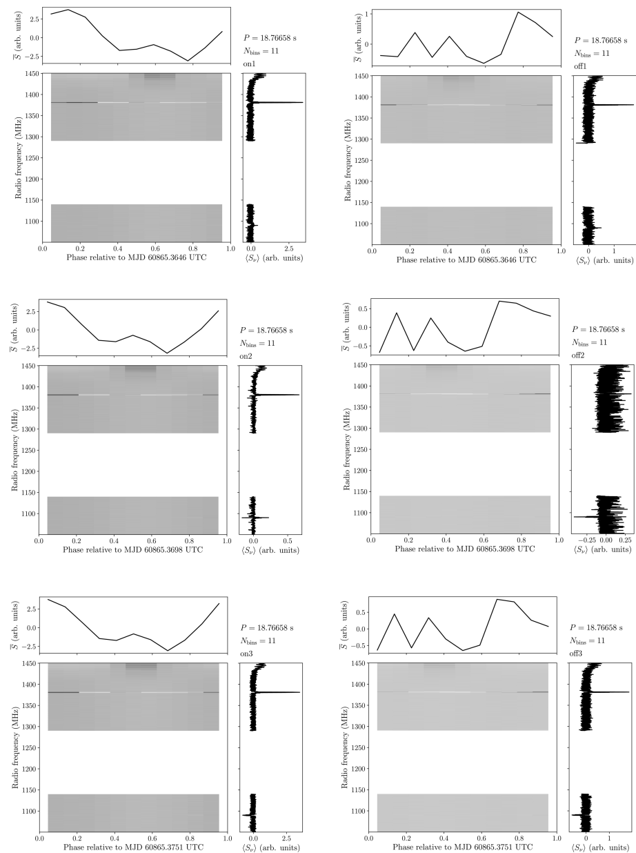
Figure 18. from Jian-Kang Li et al 2026 Astron. J. 171 doi:10.3847/1538-3881/ae28cc https://dx.doi.org/10.3847/1538-3881/ae28cc © 2026. The Author(s). Published by the American Astronomical Society.
