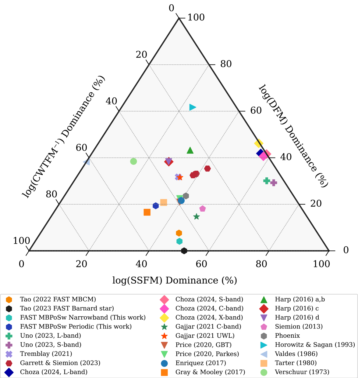
Figure 14. from Jian-Kang Li et al 2026 Astron. J. 171 doi:10.3847/1538-3881/ae28cc https://dx.doi.org/10.3847/1538-3881/ae28cc © 2026. The Author(s). Published by the American Astronomical Society.
