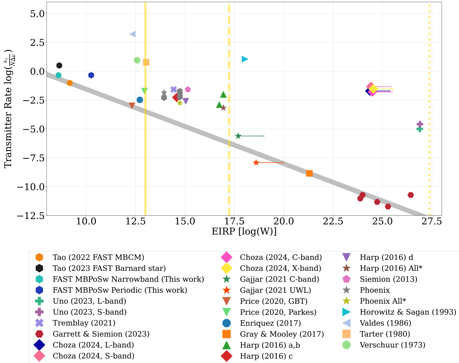
Figure 13. from Jian-Kang Li et al 2026 Astron. J. 171 doi:10.3847/1538-3881/ae28cc https://dx.doi.org/10.3847/1538-3881/ae28cc © 2026. The Author(s). Published by the American Astronomical Society.
