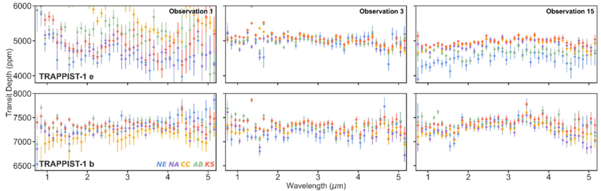
Figure 9. from Natalie H. Allen et al 2026 Astron. J. 171 doi:10.3847/1538-3881/ae28cb https://dx.doi.org/10.3847/1538-3881/ae28cb © 2026. The Author(s). Published by the American Astronomical Society.
