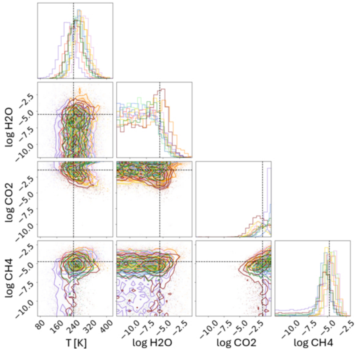
Figure 2. from Natalie H. Allen et al 2026 Astron. J. 171 doi:10.3847/1538-3881/ae28cb https://dx.doi.org/10.3847/1538-3881/ae28cb © 2026. The Author(s). Published by the American Astronomical Society.
