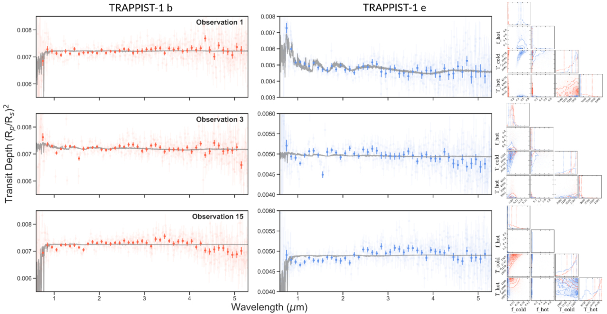
Figure 13. from Natalie H. Allen et al 2026 Astron. J. 171 doi:10.3847/1538-3881/ae28cb https://dx.doi.org/10.3847/1538-3881/ae28cb © 2026. The Author(s). Published by the American Astronomical Society.
