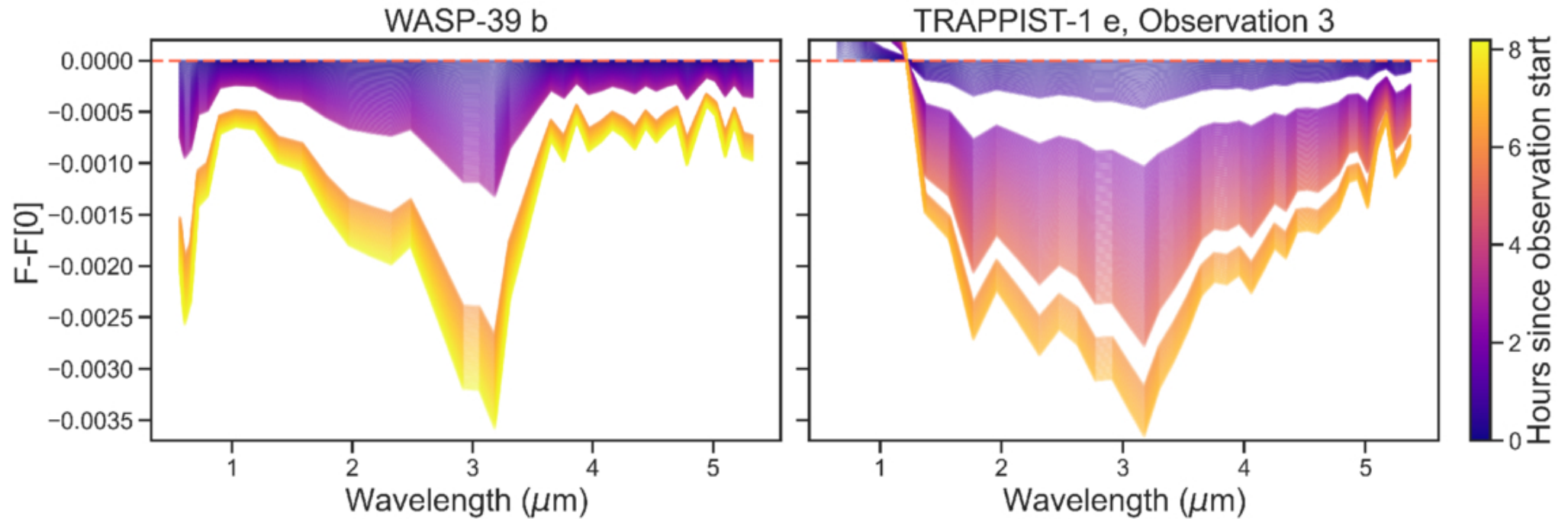
Figure 12. from Natalie H. Allen et al 2026 Astron. J. 171 doi:10.3847/1538-3881/ae28cb https://dx.doi.org/10.3847/1538-3881/ae28cb © 2026. The Author(s). Published by the American Astronomical Society.
