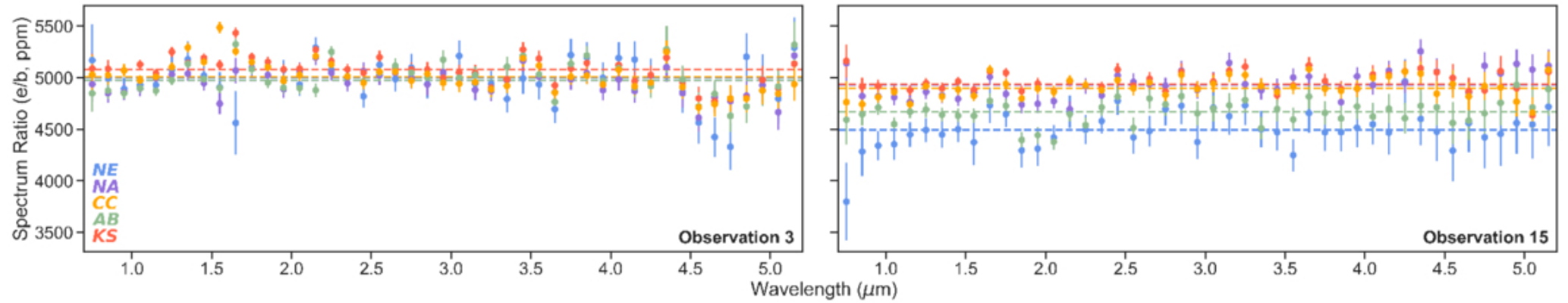
Figure 10. from Natalie H. Allen et al 2026 Astron. J. 171 doi:10.3847/1538-3881/ae28cb https://dx.doi.org/10.3847/1538-3881/ae28cb © 2026. The Author(s). Published by the American Astronomical Society.
