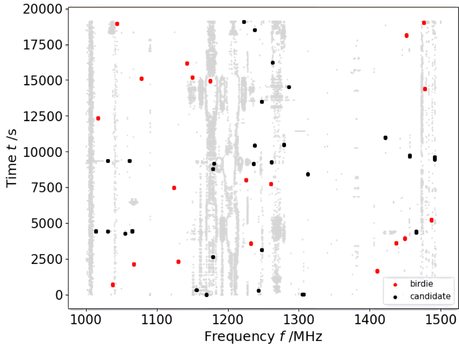
Figure 7. from Li-Li Zhao et al 2026 Astron. J. 171 doi:10.3847/1538-3881/ae28ca https://dx.doi.org/10.3847/1538-3881/ae28ca © 2026. The Author(s). Published by the American Astronomical Society.
