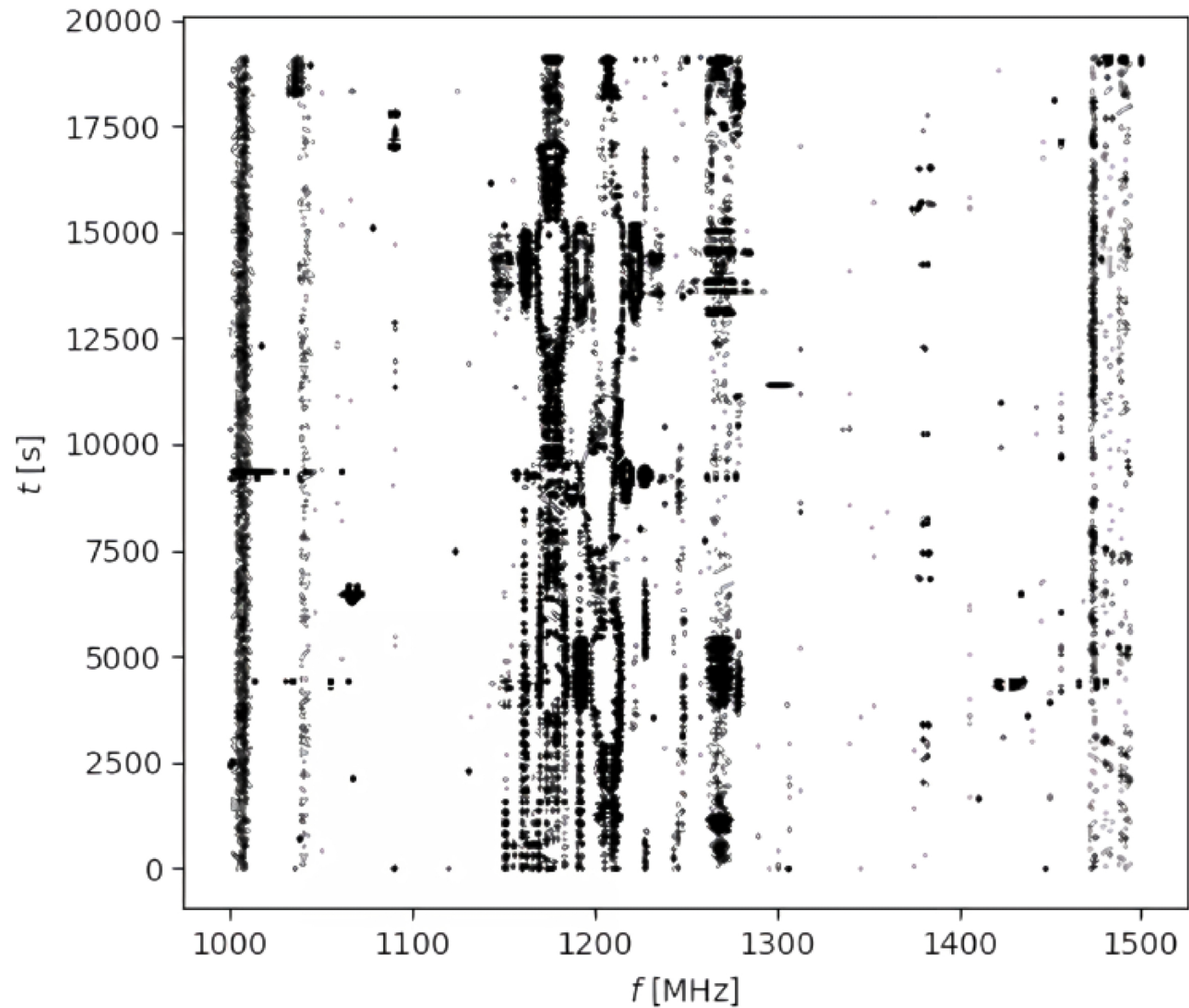
Figure 2. from Li-Li Zhao et al 2026 Astron. J. 171 doi:10.3847/1538-3881/ae28ca https://dx.doi.org/10.3847/1538-3881/ae28ca © 2026. The Author(s). Published by the American Astronomical Society.
