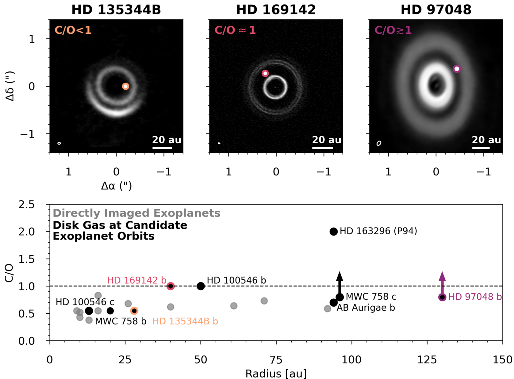
Figure 9. from Alice S. Booth et al 2026 Astron. J. 171 doi:10.3847/1538-3881/ae286b https://dx.doi.org/10.3847/1538-3881/ae286b © 2026. The Author(s). Published by the American Astronomical Society.
