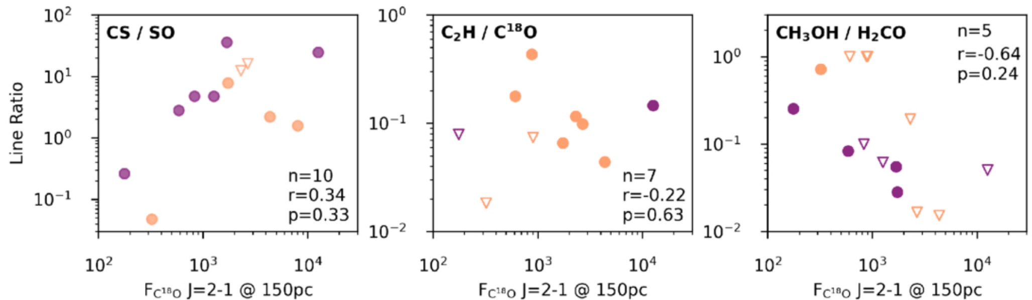
Figure 8. from Alice S. Booth et al 2026 Astron. J. 171 doi:10.3847/1538-3881/ae286b https://dx.doi.org/10.3847/1538-3881/ae286b © 2026. The Author(s). Published by the American Astronomical Society.
