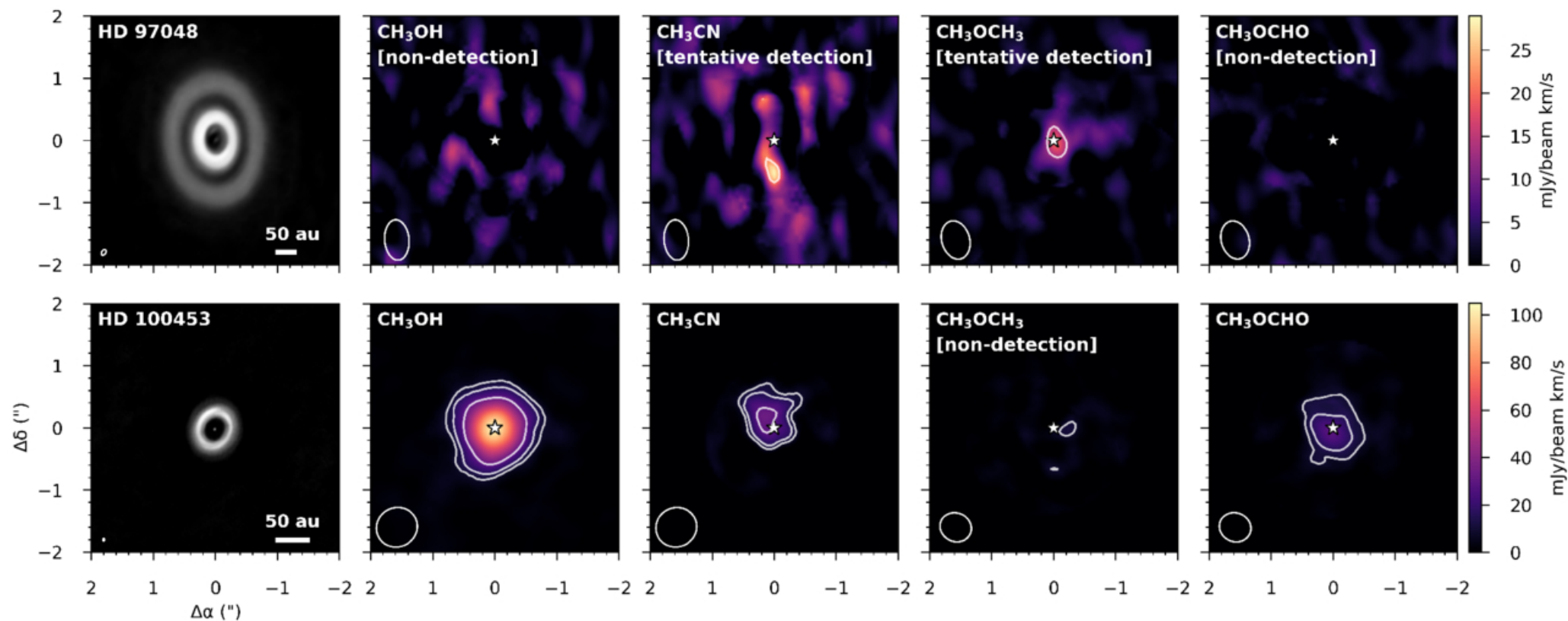
Figure 5. from Alice S. Booth et al 2026 Astron. J. 171 doi:10.3847/1538-3881/ae286b https://dx.doi.org/10.3847/1538-3881/ae286b © 2026. The Author(s). Published by the American Astronomical Society.
