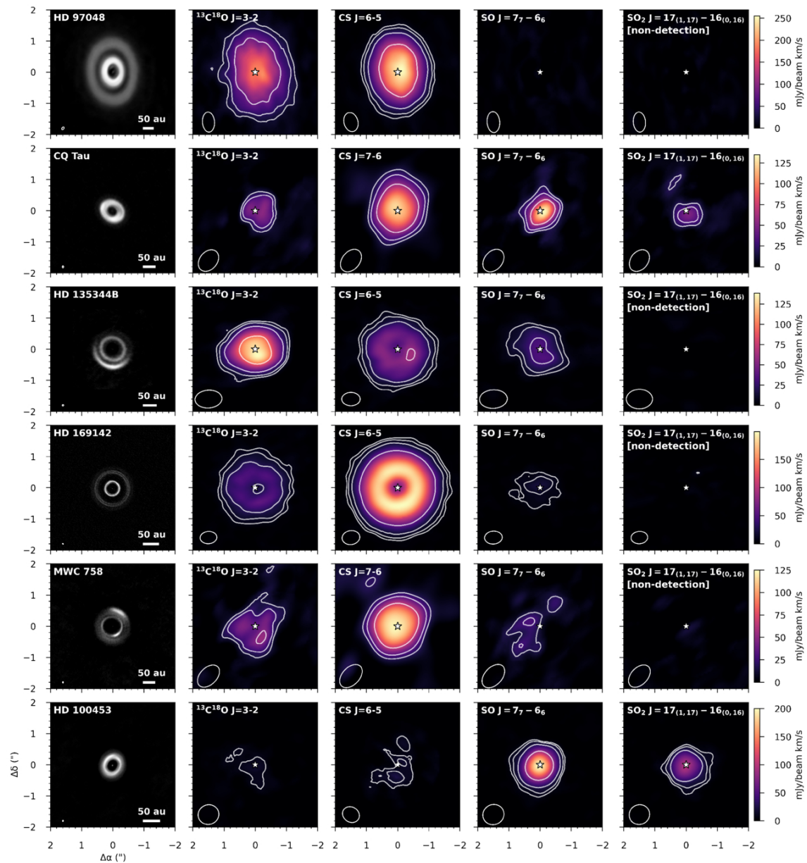
Figure 2. from Alice S. Booth et al 2026 Astron. J. 171 doi:10.3847/1538-3881/ae286b https://dx.doi.org/10.3847/1538-3881/ae286b © 2026. The Author(s). Published by the American Astronomical Society.
