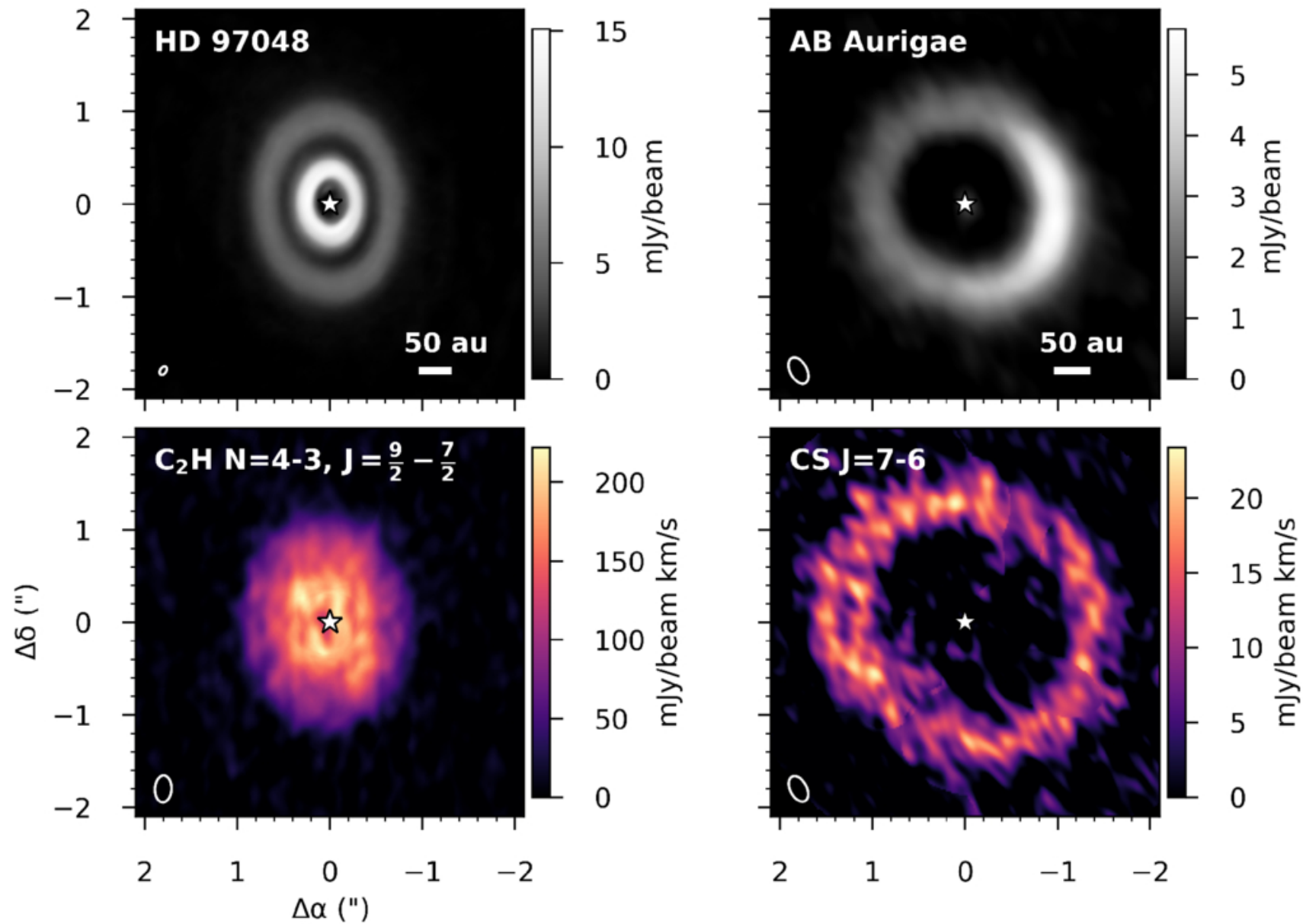
Figure 11. from Alice S. Booth et al 2026 Astron. J. 171 doi:10.3847/1538-3881/ae286b https://dx.doi.org/10.3847/1538-3881/ae286b © 2026. The Author(s). Published by the American Astronomical Society.
