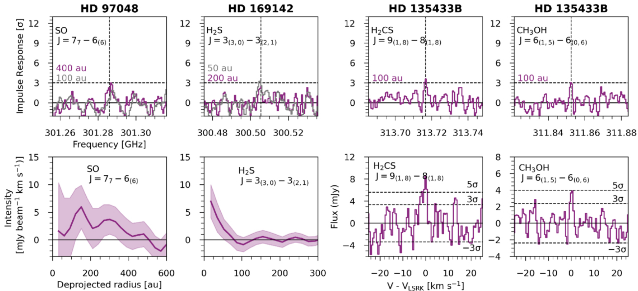
Figure 10. from Alice S. Booth et al 2026 Astron. J. 171 doi:10.3847/1538-3881/ae286b https://dx.doi.org/10.3847/1538-3881/ae286b © 2026. The Author(s). Published by the American Astronomical Society.
