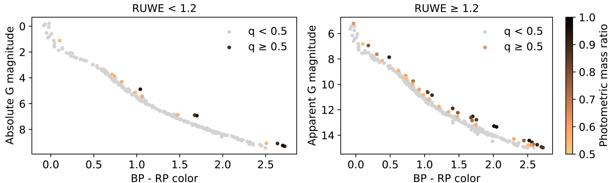
Figure 9. from Dmitry Chulkov 2026 Astron. J. 171 doi:10.3847/1538-3881/ae284e https://dx.doi.org/10.3847/1538-3881/ae284e © 2026. The Author(s). Published by the American Astronomical Society.
