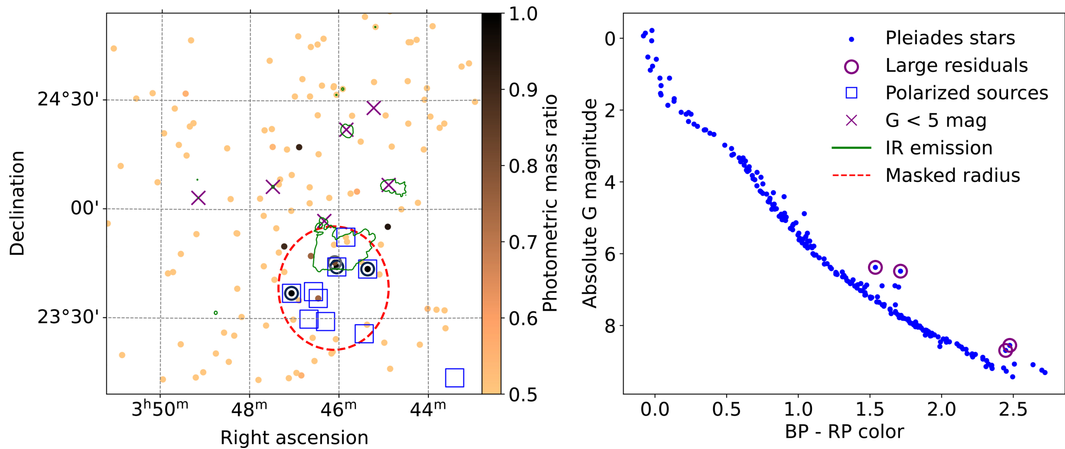
Figure 7. from Dmitry Chulkov 2026 Astron. J. 171 doi:10.3847/1538-3881/ae284e https://dx.doi.org/10.3847/1538-3881/ae284e © 2026. The Author(s). Published by the American Astronomical Society.
